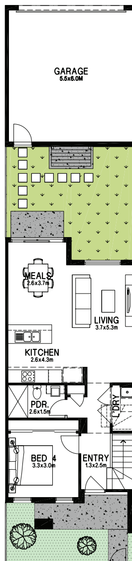
GROUND FLOOR
